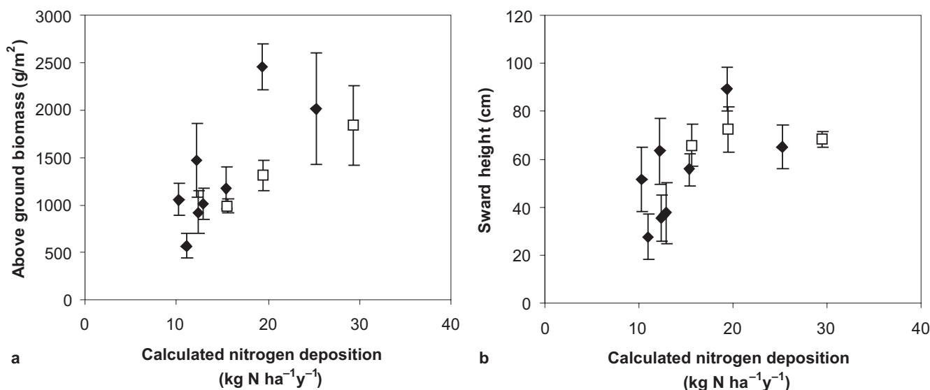
Fig. 1 Data from the mobile and semi-fixed dunes in relation to N inputs showing (a) above ground biomass ( \text{g m}^{-2} ) and (b) sward height
