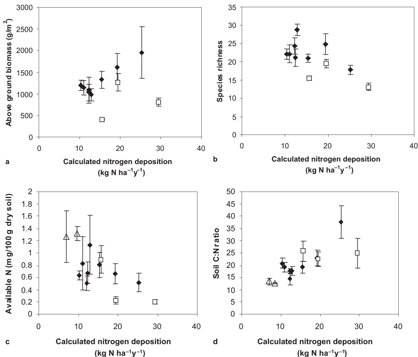
Fig. 2 Data from the fixed dunes and dune grasslands in relation to N inputs showing (a) above ground biomass ( \text{g m}^{-2} ), (b) species richness, (c) soil available N ( \text{mg } 100 \text{ g dry soil}^{-1} ), and (d) soil C:N ratio. Filled
